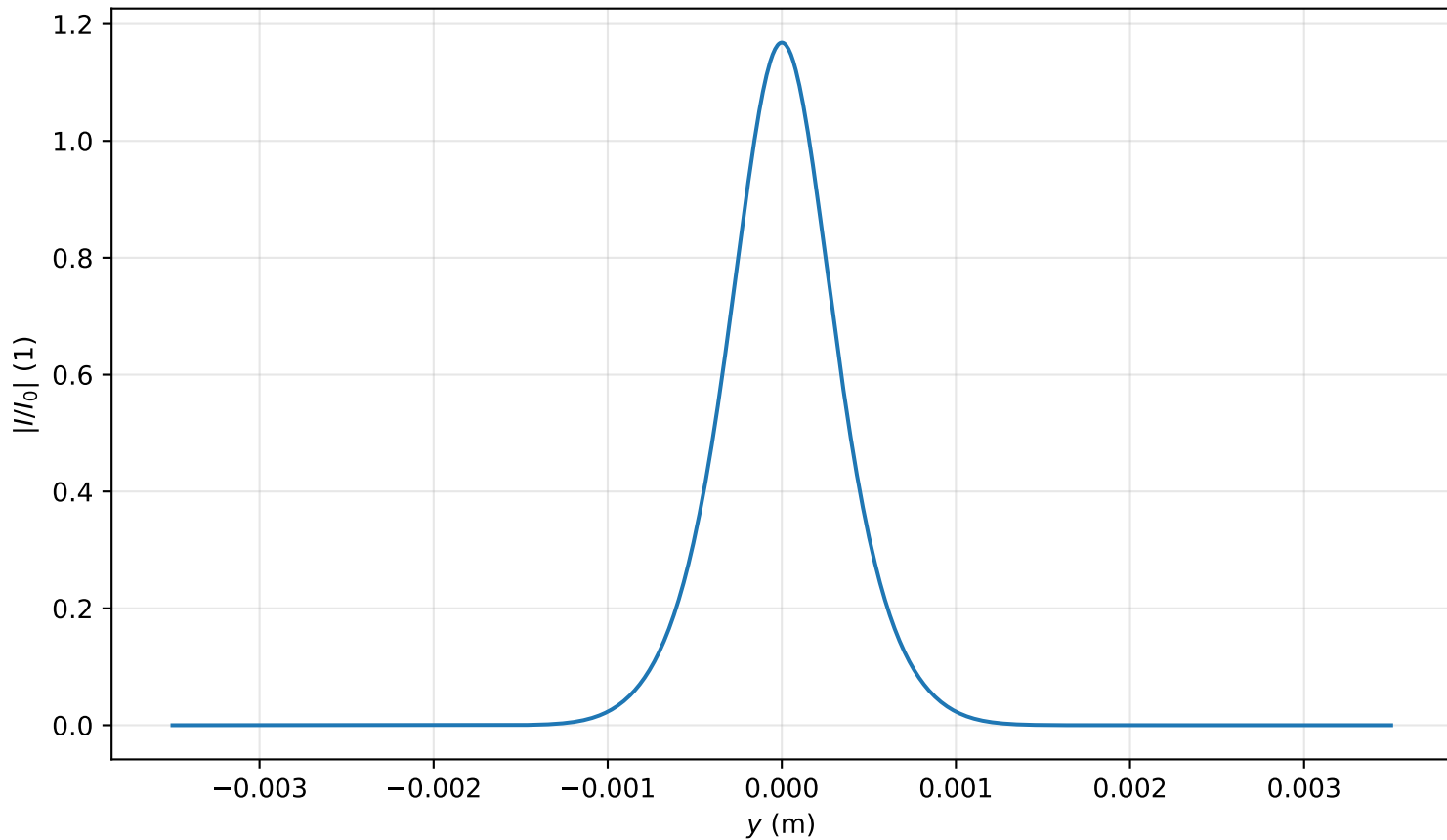
Intensity profile I(x=0, y, z=0.796)/I_0 , P_{in}=0.7P_{cr} , artificial time
